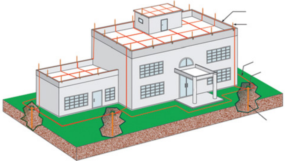
Bonding Strip Franklin Rod
